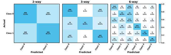
Fig. 13: Normalized confusion matrices for the multimodal GRU-CNN baseline.
