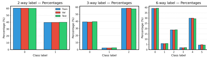
Fig. 1: Label distributions across train/validation/test.
