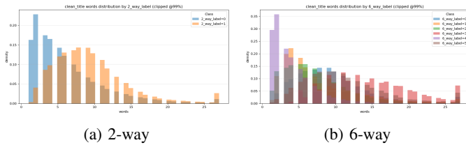
Fig. 3: Title word-count distributions.
