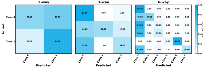
Fig. 11: Normalized confusion matrices for the image-only baseline across 2-way, 3-way, and 6-way classification.
